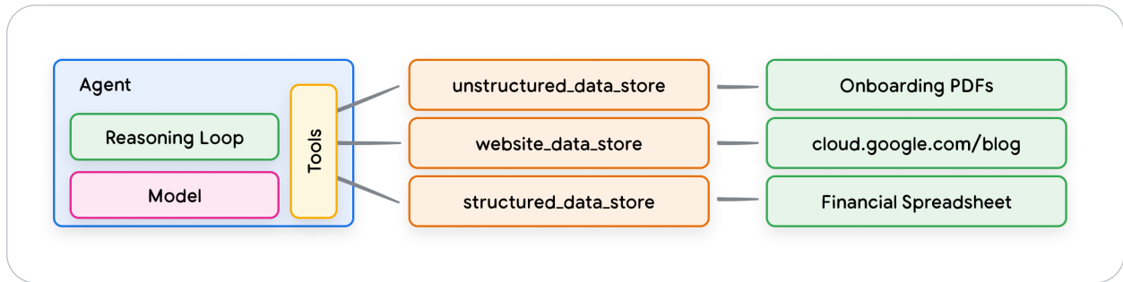
Figure 12. 1-to-many relationship between agents and data stores, which can represent various types of pre-indexed data
